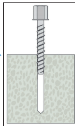
Insert anchor into concrete using suitable impact wrench
