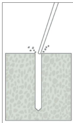
Clean hole by blowing to remove drilling debris and dust
